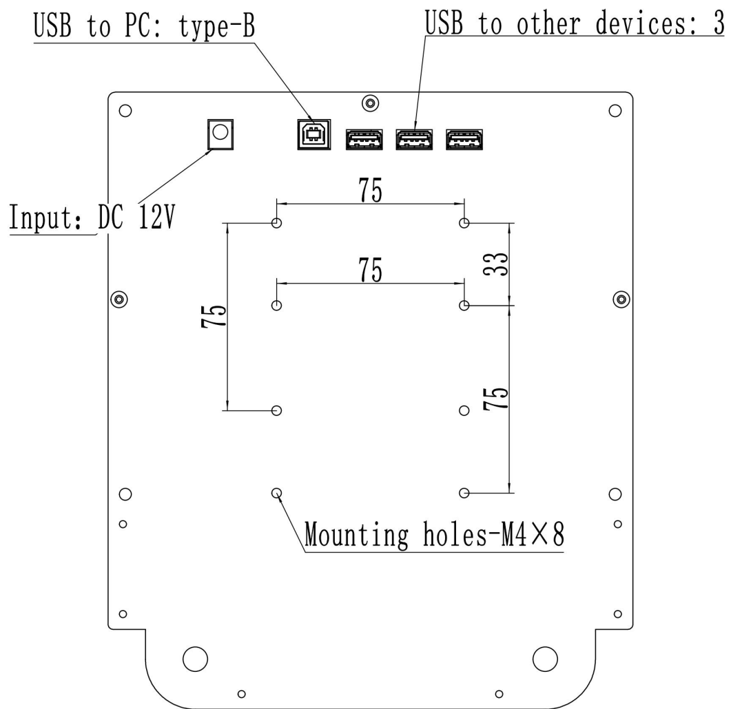
Mounting dimensions
